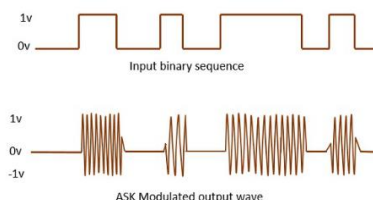
Digital Modulation
