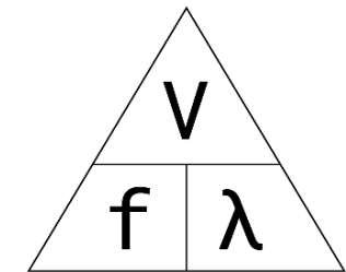
Wavelength Triangle
