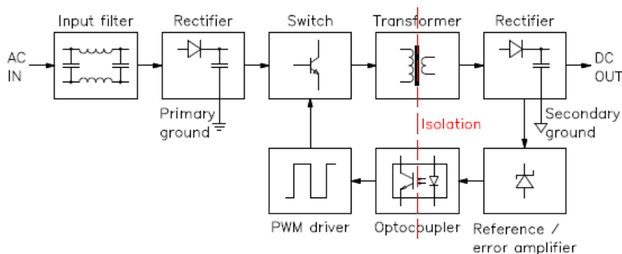
Switch mode power supply block diagram
